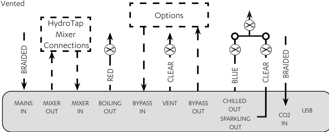
All-in-One Classic Vented
