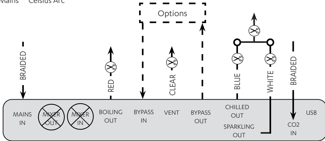
All-in-One Classic Mains All-in-One Celsius Arc
