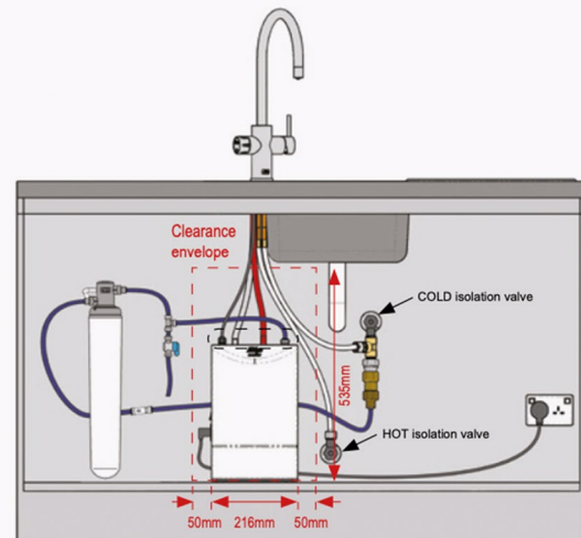
FILTERED BOILING | HOT & COLD HYDROTAP
