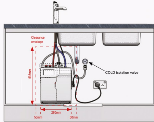
FILTERED BOILING | CHILLED
